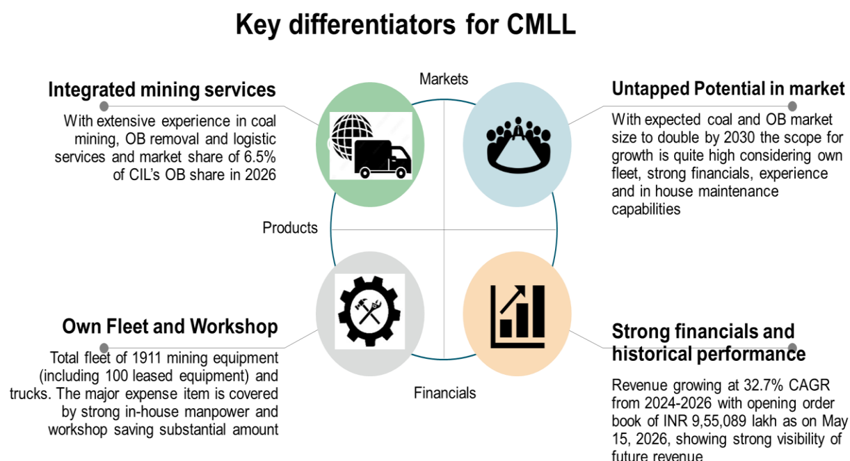
Figure 0.81 Key differentiators
